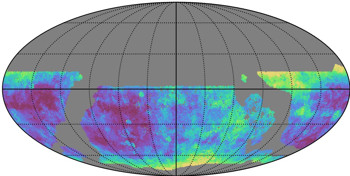
too_elab_r8_d2_ugrizy_v3.4_10yrs WFD g band: Median seeingEff
