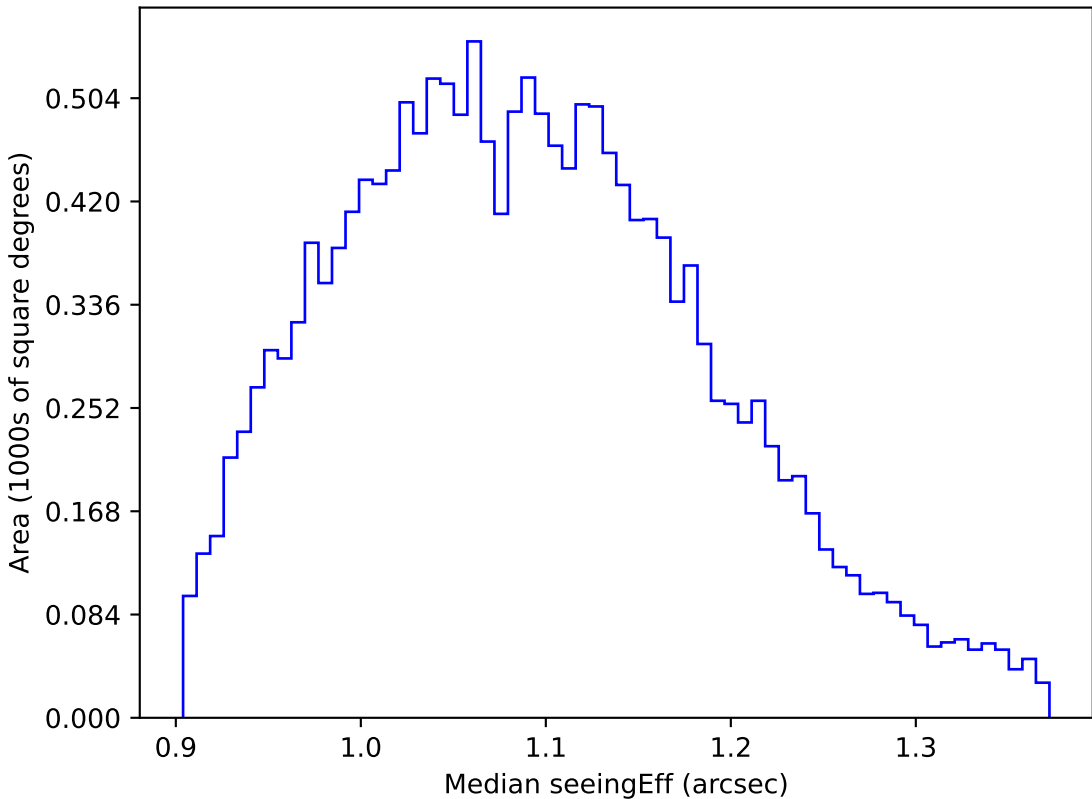
too_elab_r8_d2_ugrizy_v3.4_10yrs WFD g band: Median seeingEff
