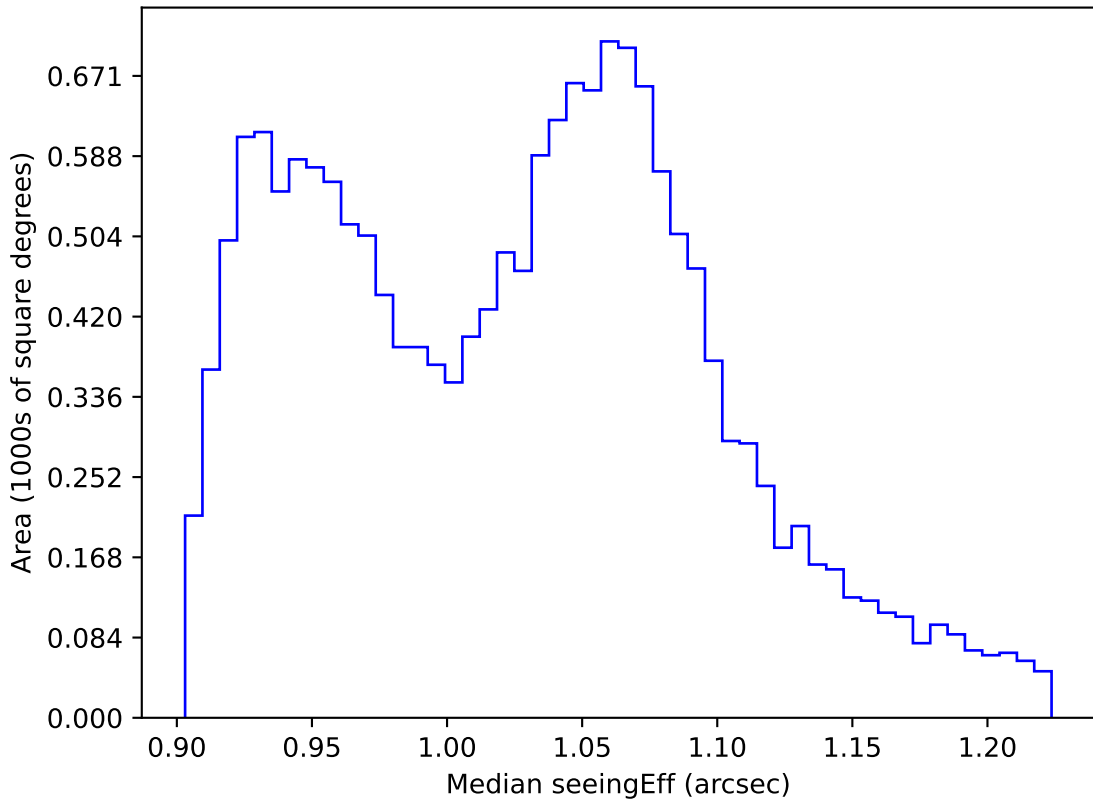
too_elab_r8_d2_ugrizy_v3.4_10yrs WFD all bands: Median seeingEff
