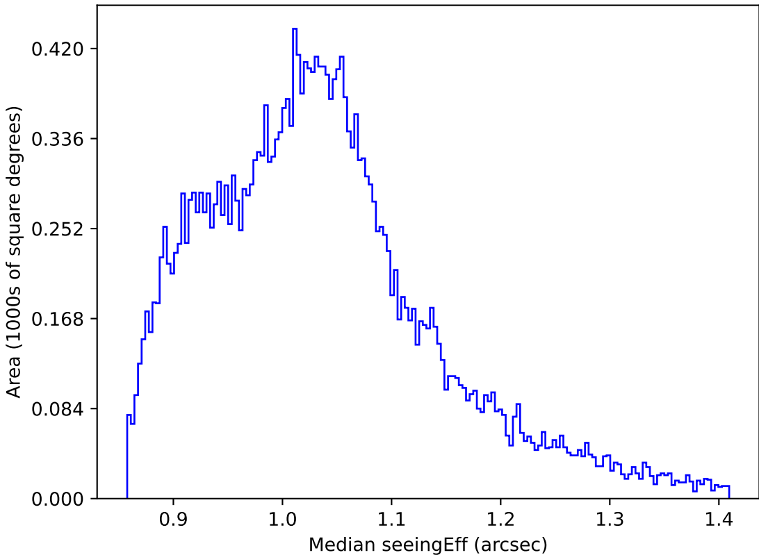
too_elab_r8_d2_ugrizy_v3.4_10yrs All sky z band: Median seeingEff
