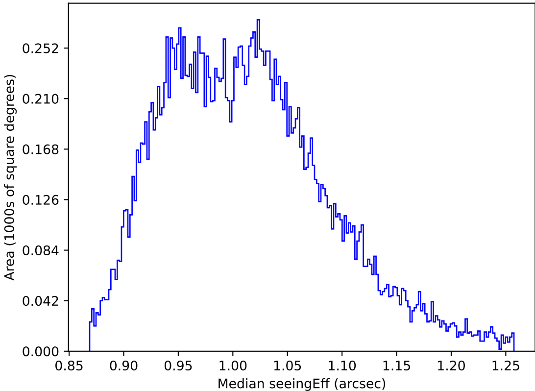
too_elab_r8_d2_ugrizy_v3.4_10yrs All sky y band: Median seeingEff
