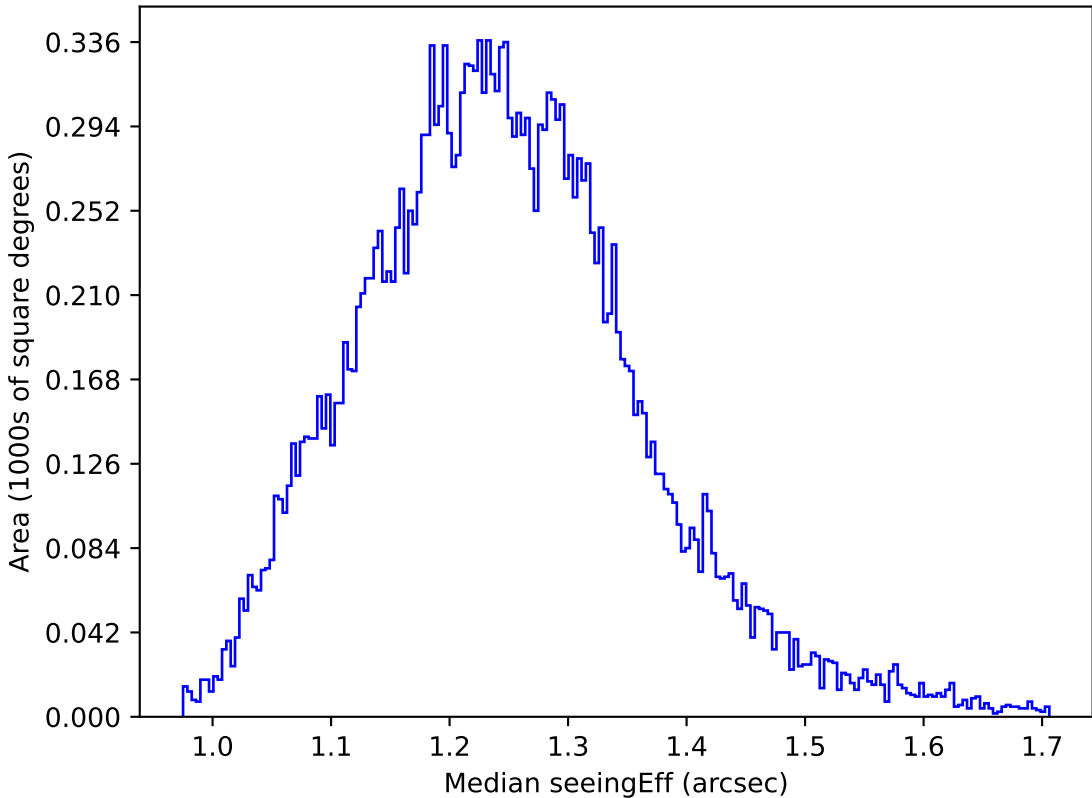
too_elab_r8_d2_ugrizy_v3.4_10yrs All sky u band: Median seeingEff
