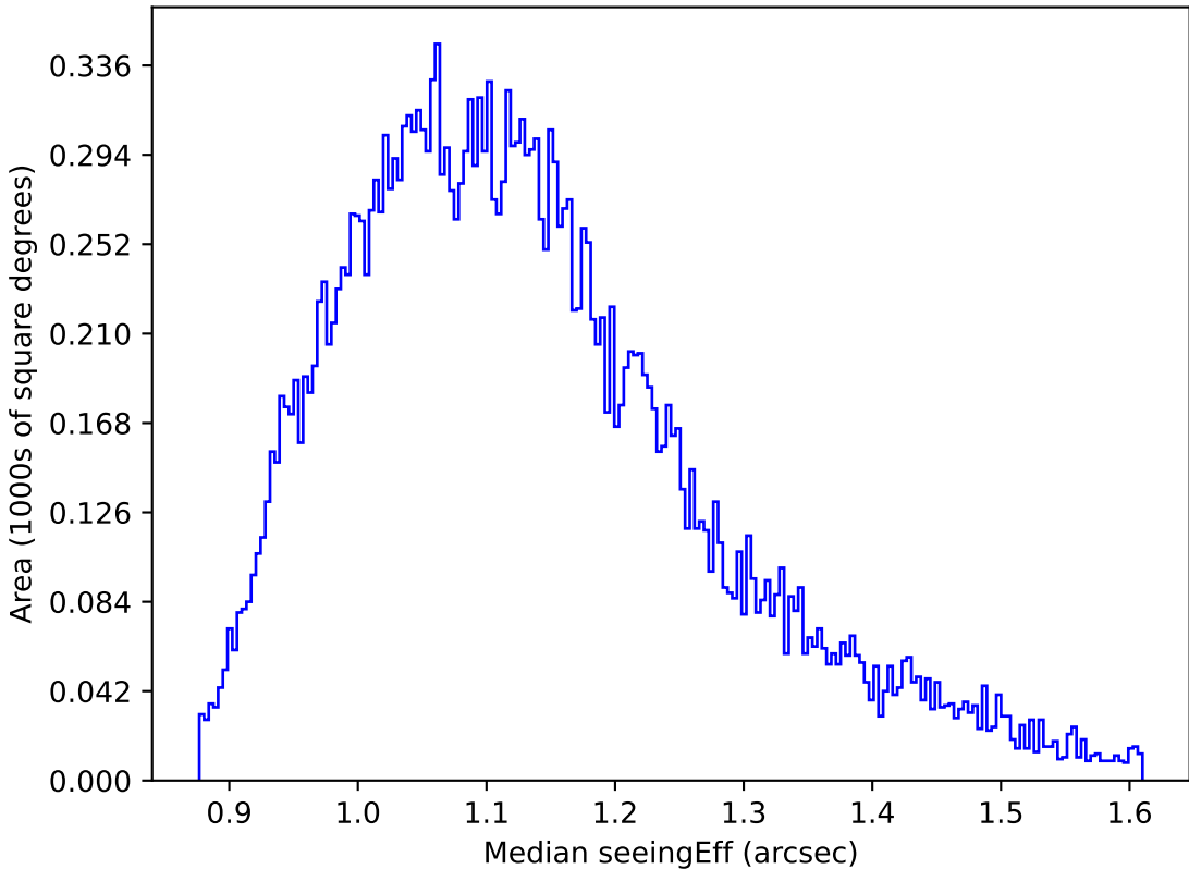
too_elab_r8_d2_ugrizy_v3.4_10yrs All sky g band: Median seeingEff
