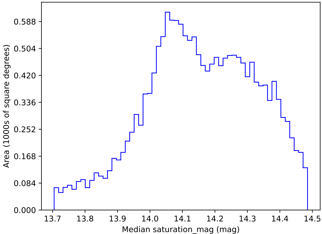
too_elab_r8_d2_ugrizy_v3.4_10yrs WFD all bands: Median saturation_mag
