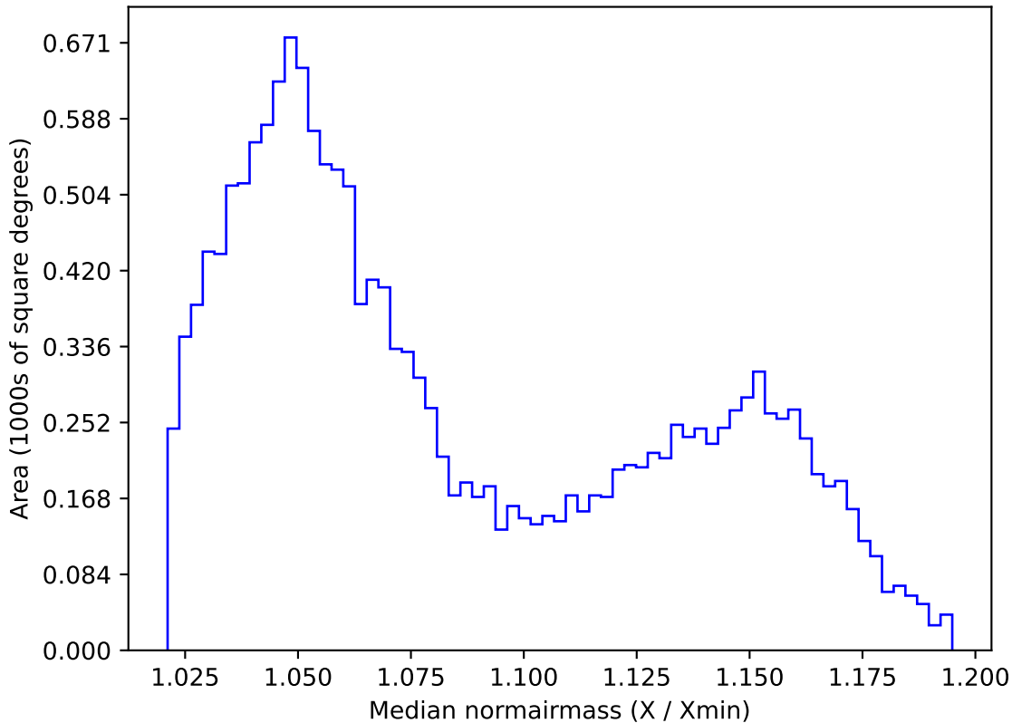
too_elab_r8_d2_ugrizy_v3.4_10yrs WFD z band: Median normairmass
