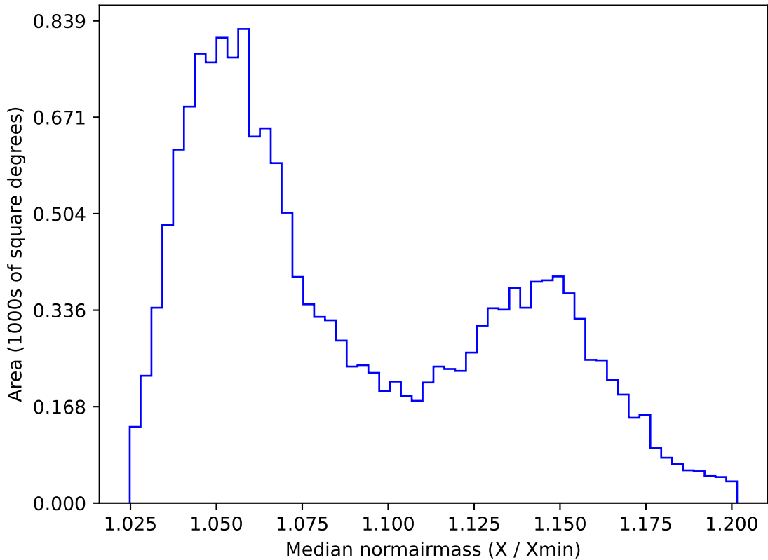
too_elab_r8_d2_ugrizy_v3.4_10yrs WFD y band: Median normairmass
