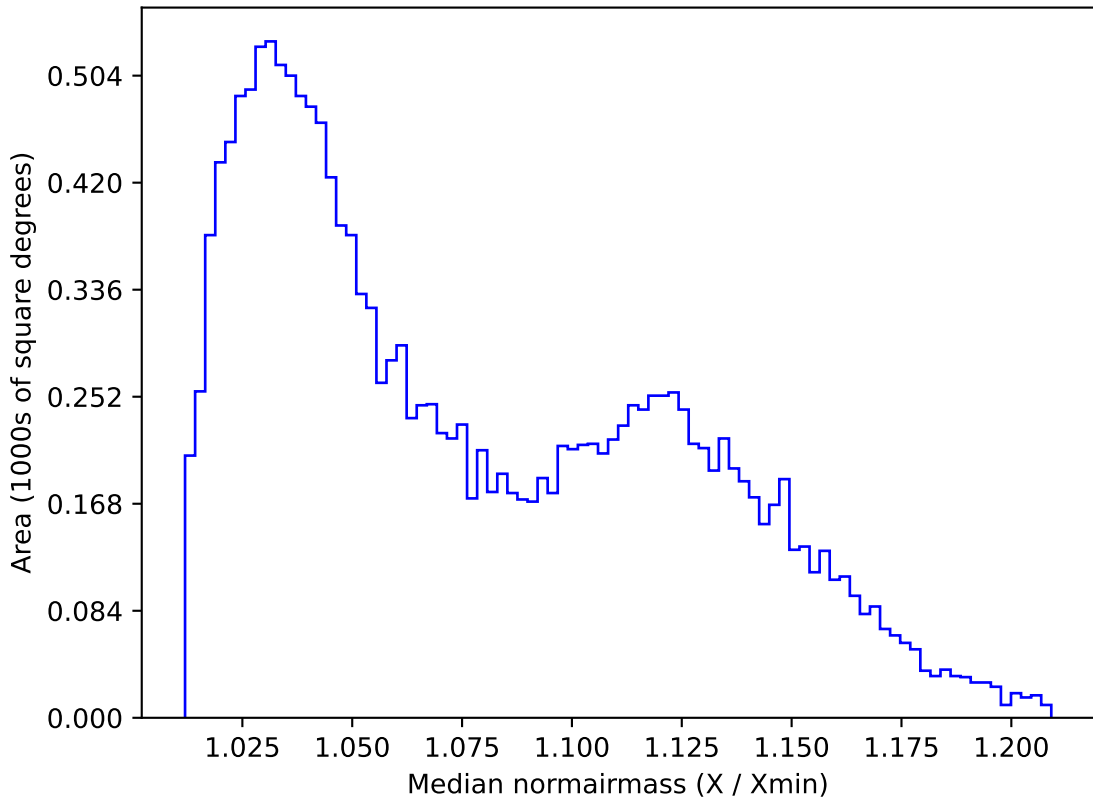
too_elab_r8_d2_ugrizy_v3.4_10yrs WFD u band: Median normairmass
