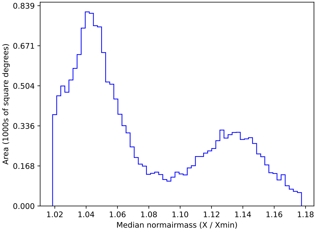
too_elab_r8_d2_ugrizy_v3.4_10yrs WFD i band: Median normairmass
