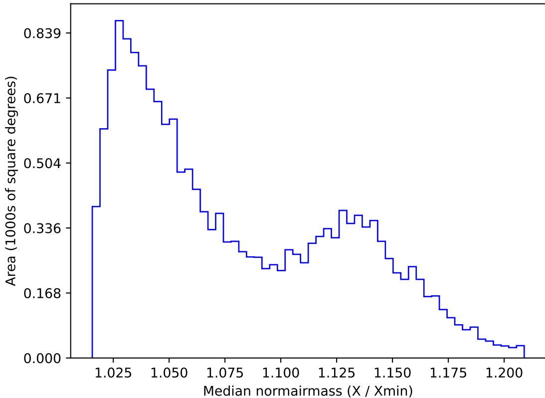
too_elab_r8_d2_ugrizy_v3.4_10yrs WFD g band: Median normairmass
