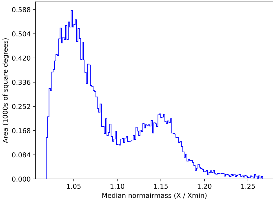
too_elab_r8_d2_ugrizy_v3.4_10yrs All sky z band: Median normairmass
