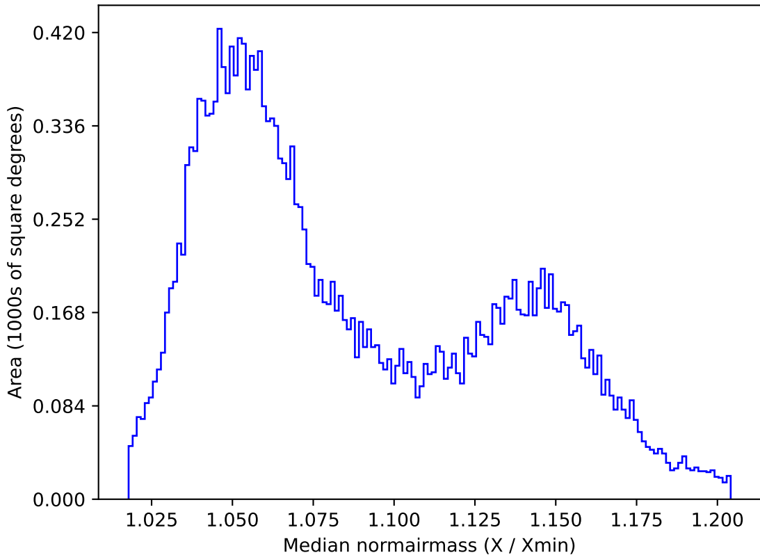
too_elab_r8_d2_ugrizy_v3.4_10yrs All sky y band: Median normairmass
