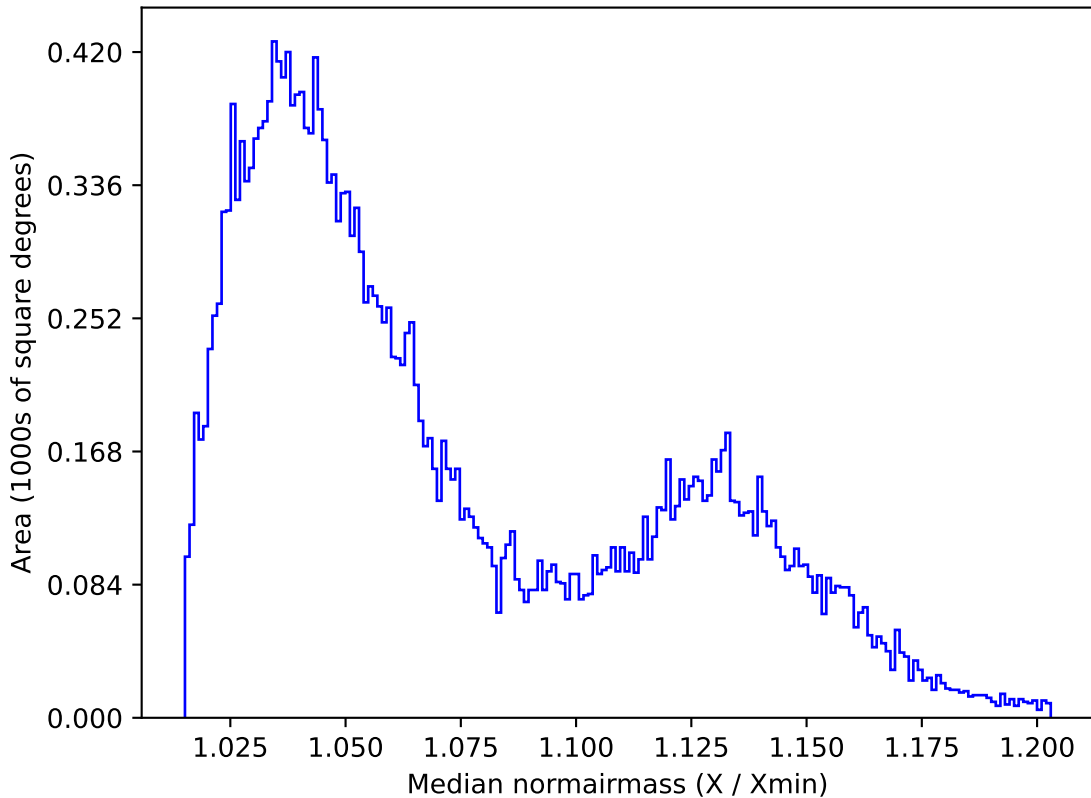
too_elab_r8_d2_ugrizy_v3.4_10yrs All sky r band: Median normairmass
