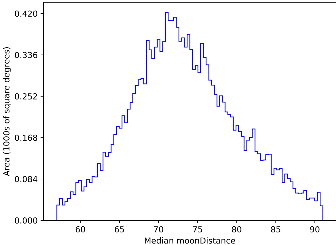
too_elab_r8_d2_ugrizy_v3.4_10yrs WFD z band: Median moonDistance
