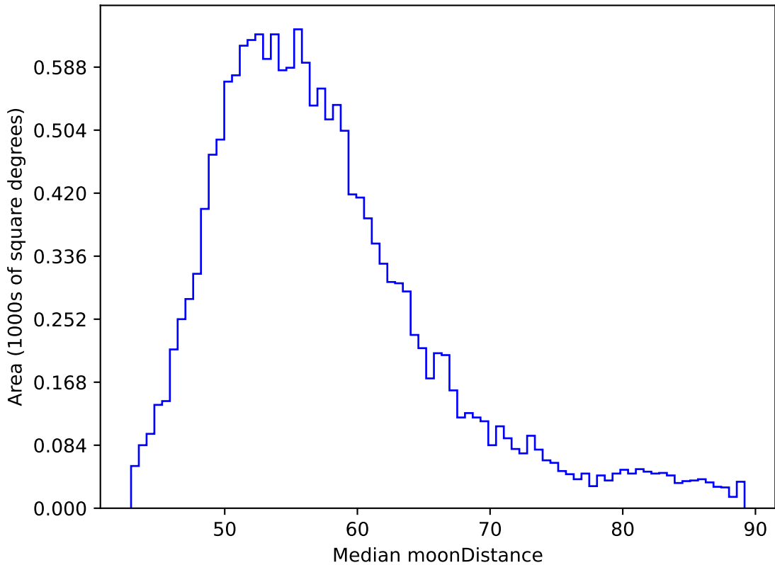
too_elab_r8_d2_ugrizy_v3.4_10yrs WFD y band: Median moonDistance
