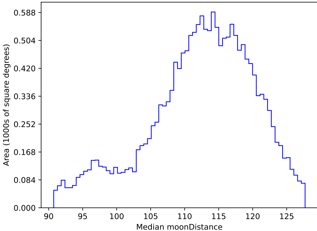
too_elab_r8_d2_ugrizy_v3.4_10yrs WFD r band: Median moonDistance
