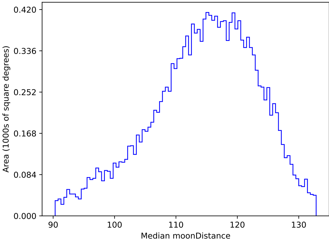
too_elab_r8_d2_ugrizy_v3.4_10yrs WFD g band: Median moonDistance
