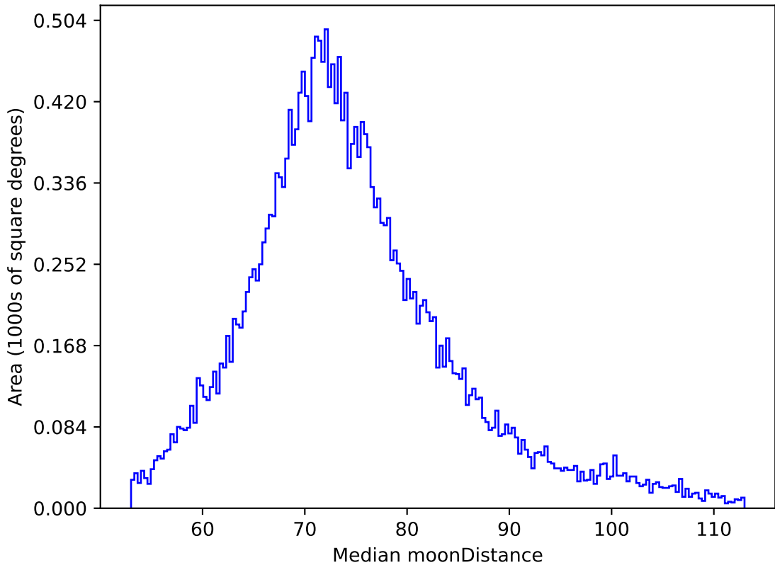
too_elab_r8_d2_ugrizy_v3.4_10yrs All sky z band: Median moonDistance
