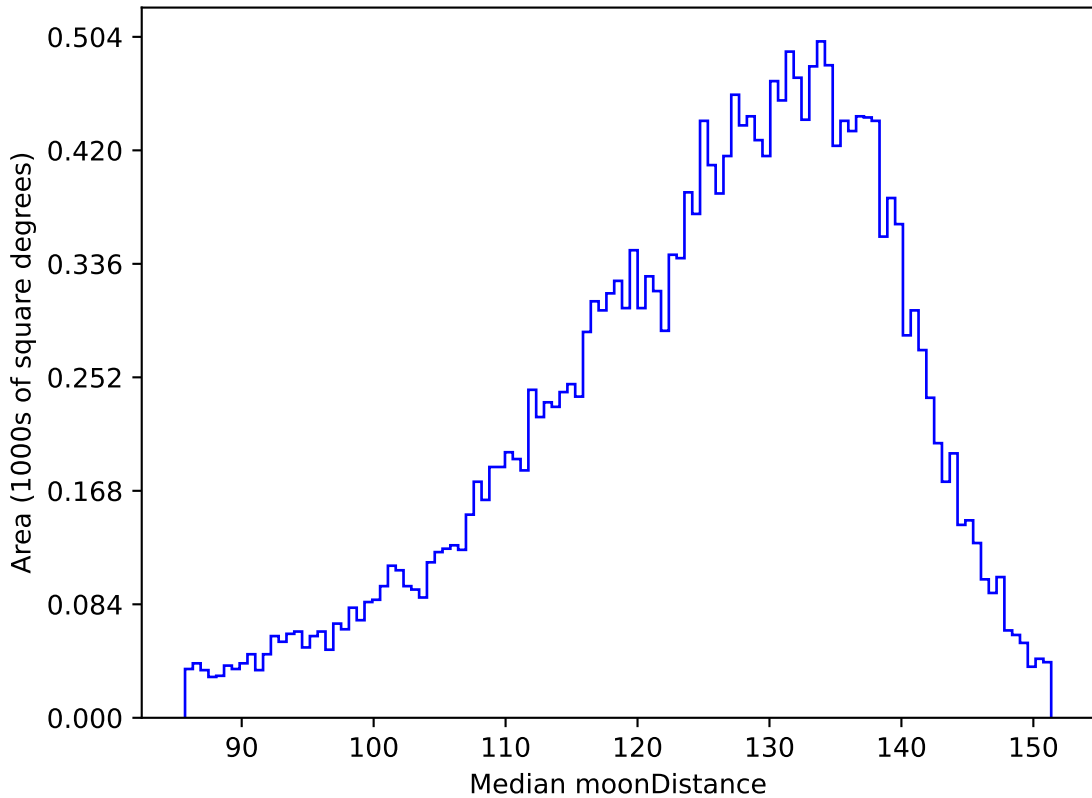
too_elab_r8_d2_ugrizy_v3.4_10yrs All sky u band: Median moonDistance
