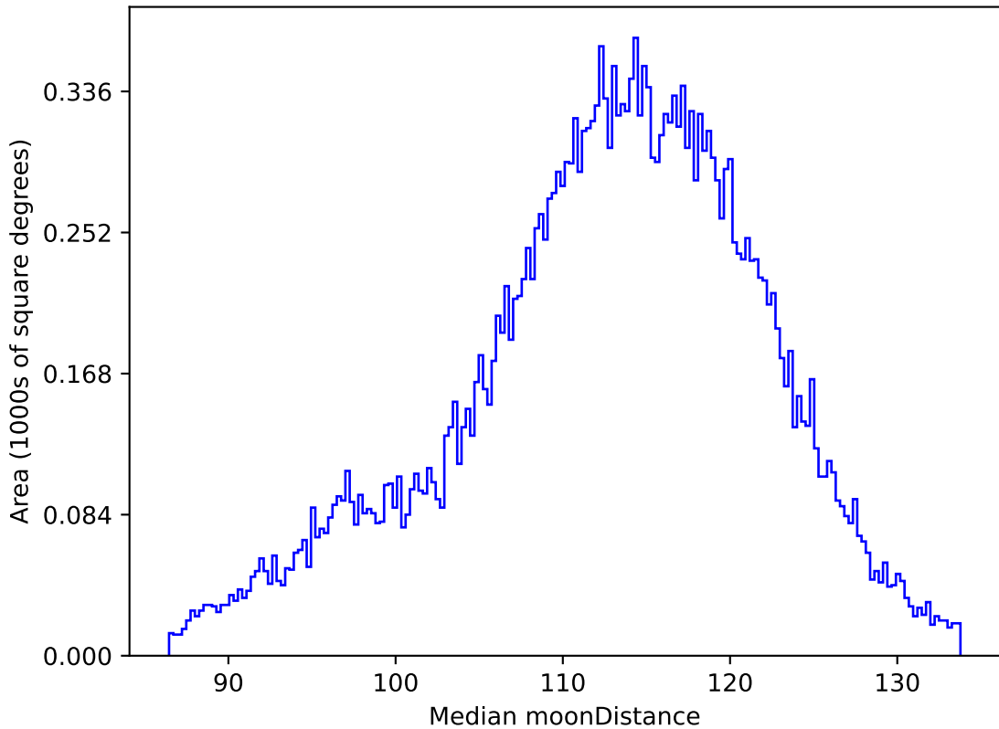
too_elab_r8_d2_ugrizy_v3.4_10yrs All sky r band: Median moonDistance
