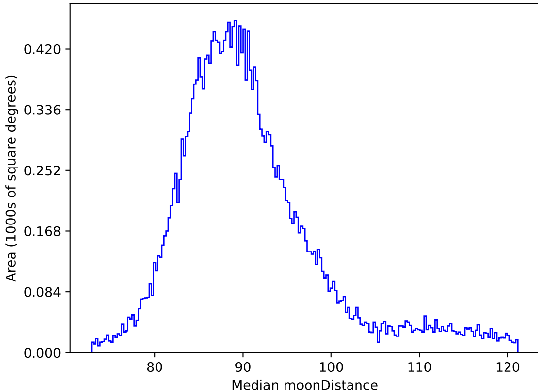
too_elab_r8_d2_ugrizy_v3.4_10yrs All sky all bands: Median moonDistance
