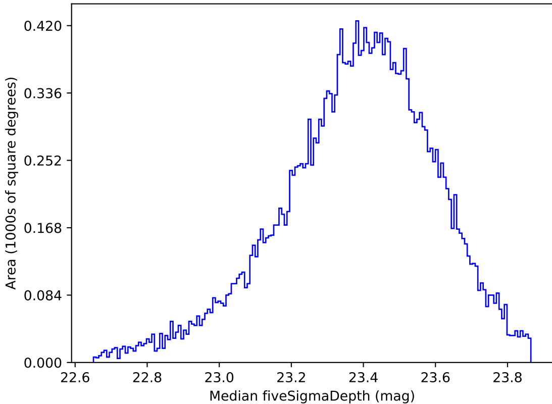
too_elab_r8_d2_ugrizy_v3.4_10yrs Yr 1 all bands: Median fiveSigmaDepth
