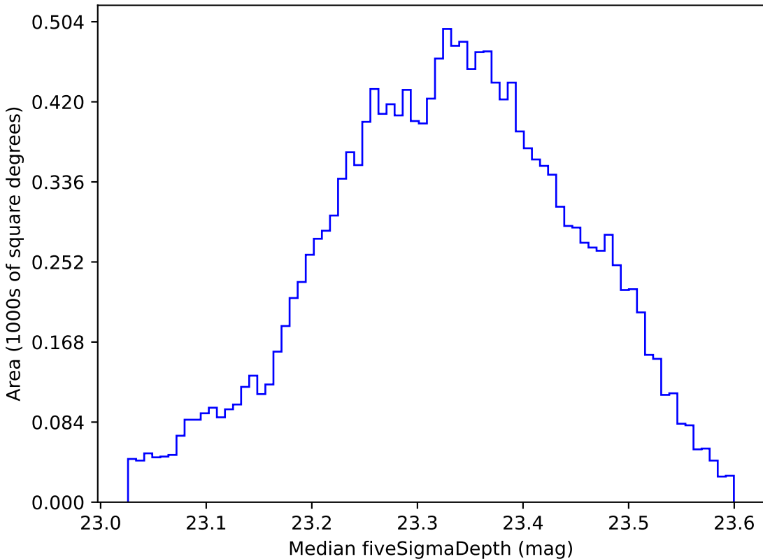
too_elab_r8_d2_ugrizy_v3.4_10yrs WFD all bands: Median fiveSigmaDepth
