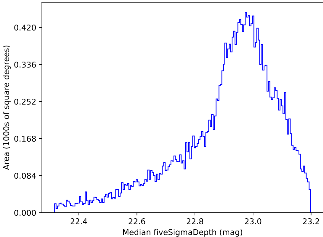
too_elab_r8_d2_ugrizy_v3.4_10yrs All sky z band: Median fiveSigmaDepth
