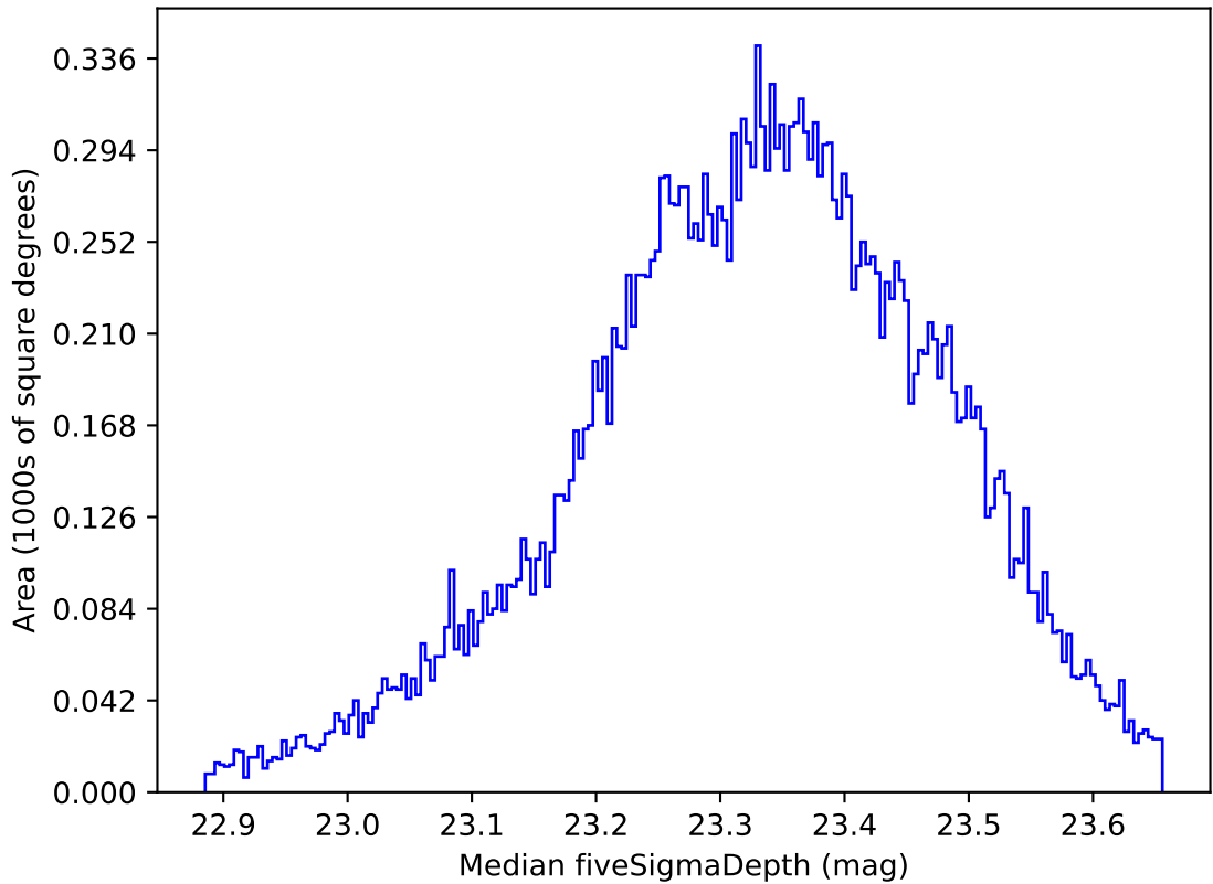
too_elab_r8_d2_ugrizy_v3.4_10yrs All sky all bands: Median fiveSigmaDepth
