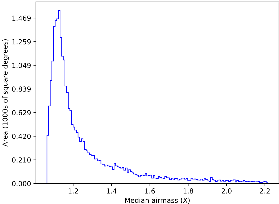
too_elab_r8_d2_ugrizy_v3.4_10yrs Yr 1 z band: Median airmass
