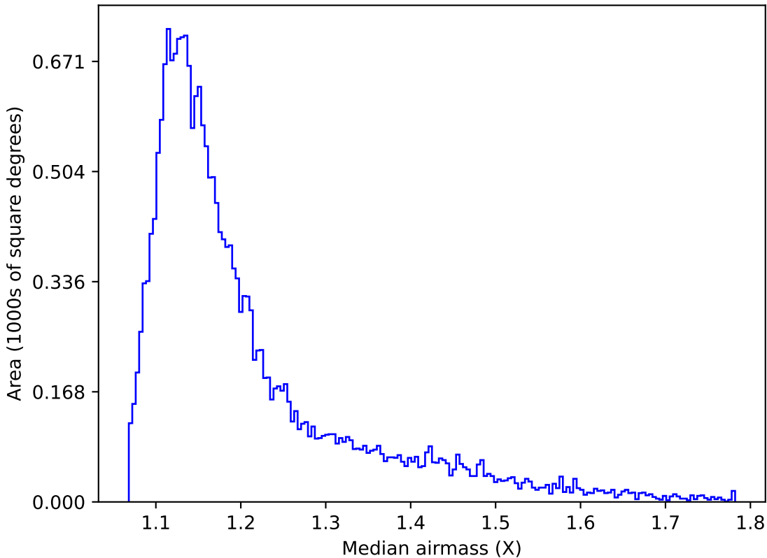
too_elab_r8_d2_ugrizy_v3.4_10yrs Yr 1 y band: Median airmass
