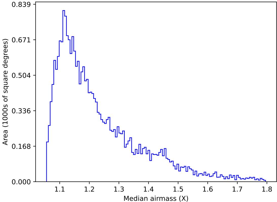
too_elab_r8_d2_ugrizy_v3.4_10yrs Yr 1 u band: Median airmass
