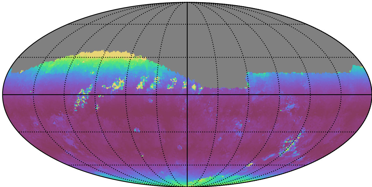
too_elab_r8_d2_ugrizy_v3.4_10yrs Yr 1 r band: Median airmass
