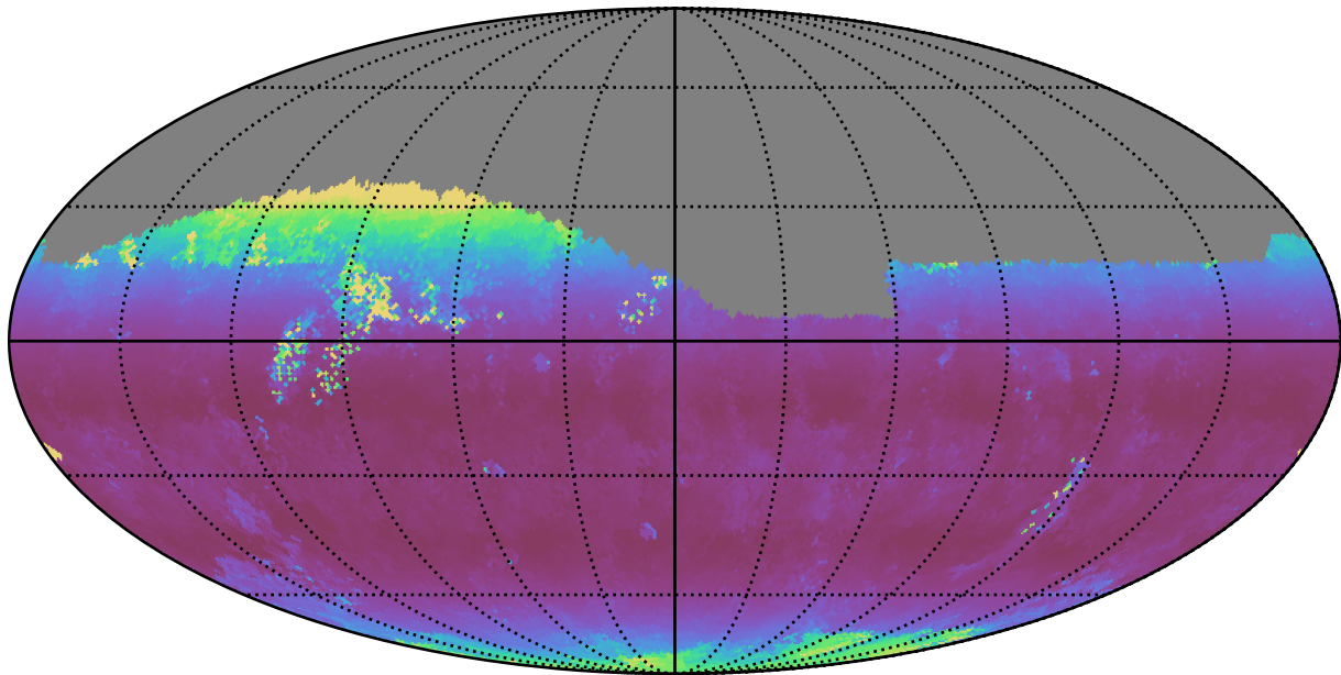
too_elab_r8_d2_ugrizy_v3.4_10yrs Yr 1 i band: Median airmass
