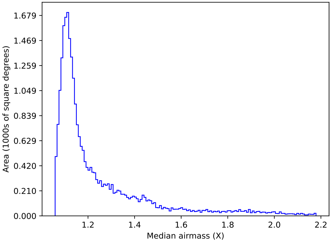
too_elab_r8_d2_ugrizy_v3.4_10yrs Yr 1 i band: Median airmass
