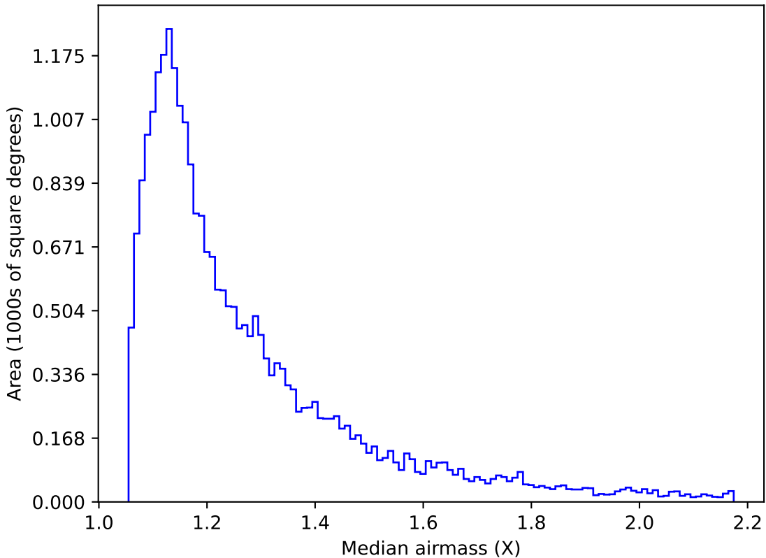
too_elab_r8_d2_ugrizy_v3.4_10yrs Yr 1 g band: Median airmass
