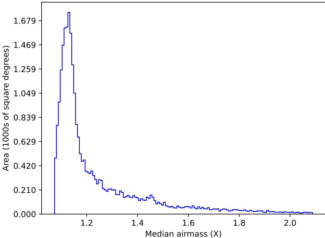
too_elab_r8_d2_ugrizy_v3.4_10yrs Yr 1 all bands: Median airmass
