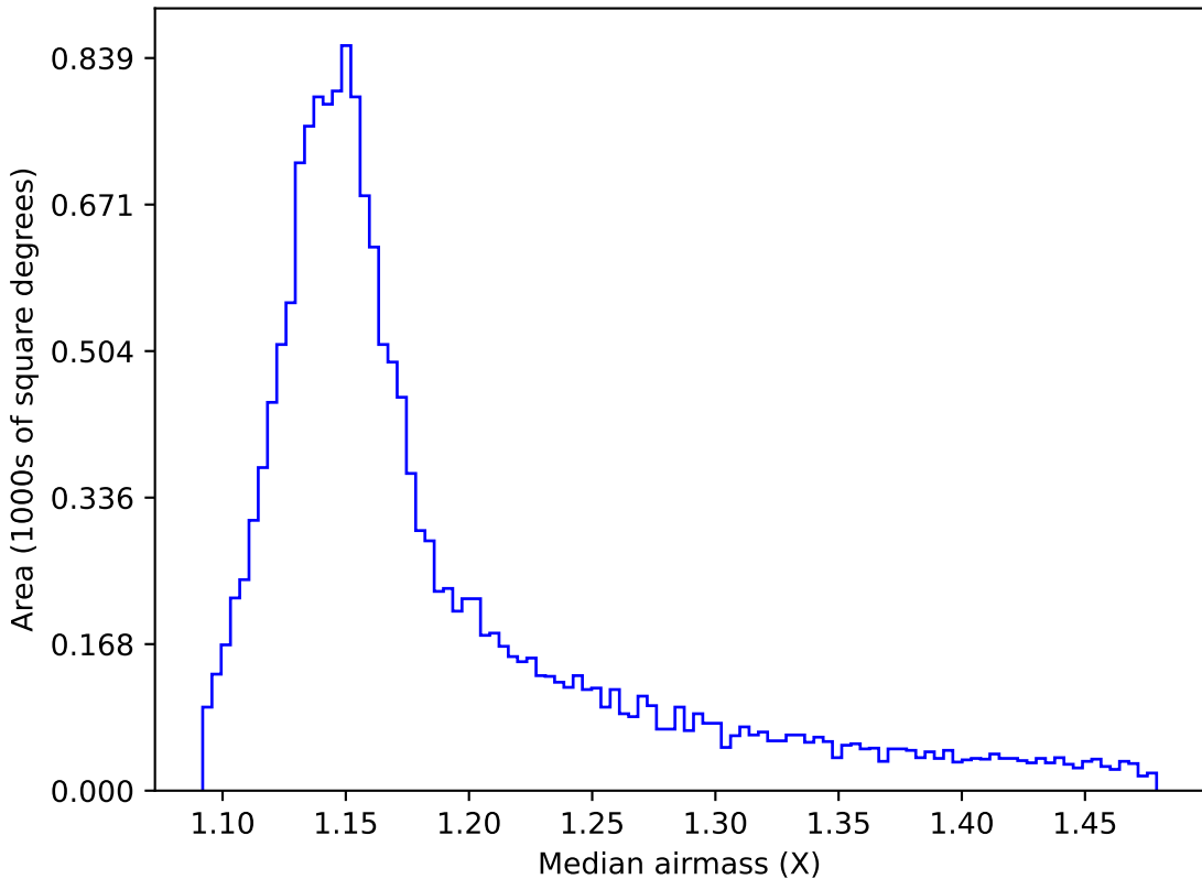
too_elab_r8_d2_ugrizy_v3.4_10yrs WFD y band: Median airmass
