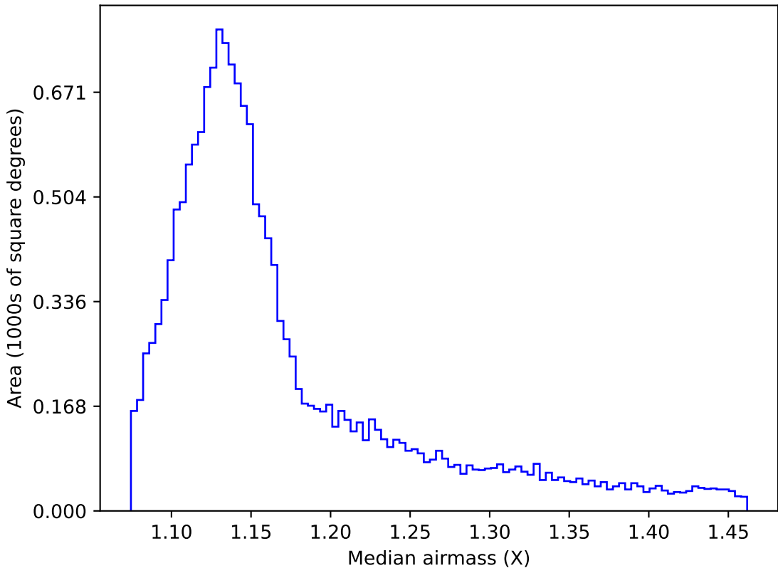
too_elab_r8_d2_ugrizy_v3.4_10yrs WFD r band: Median airmass
