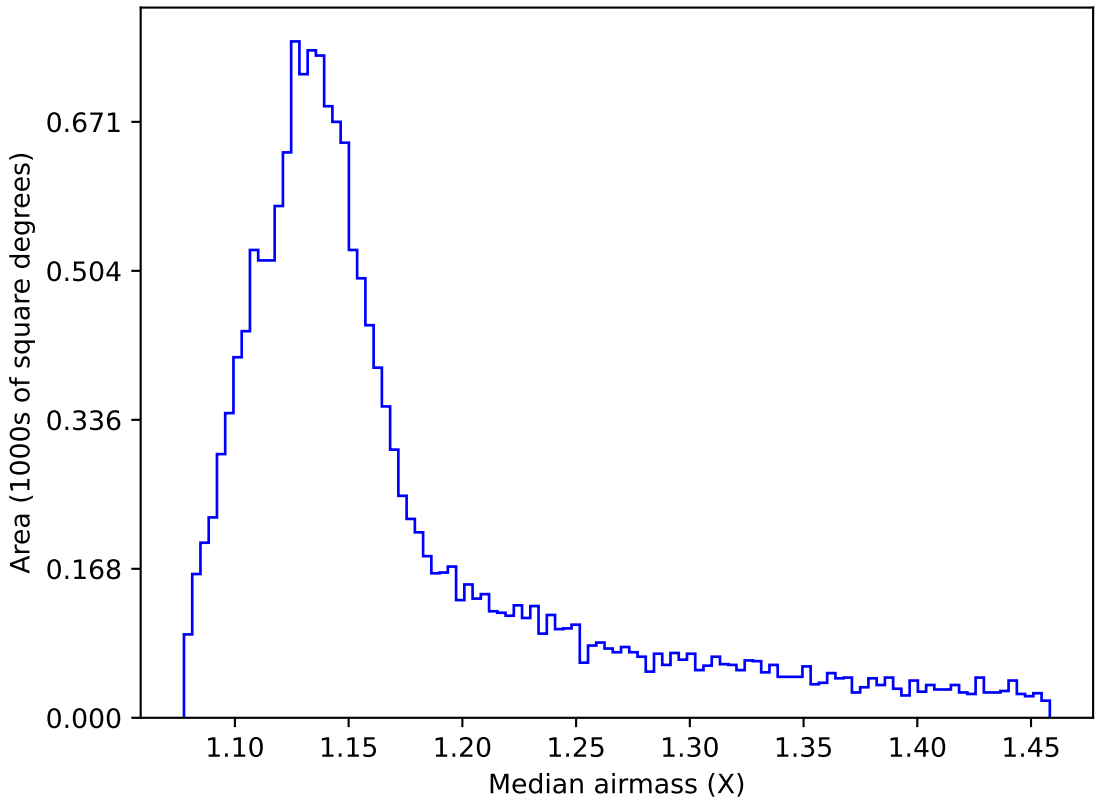
too_elab_r8_d2_ugrizy_v3.4_10yrs WFD i band: Median airmass
