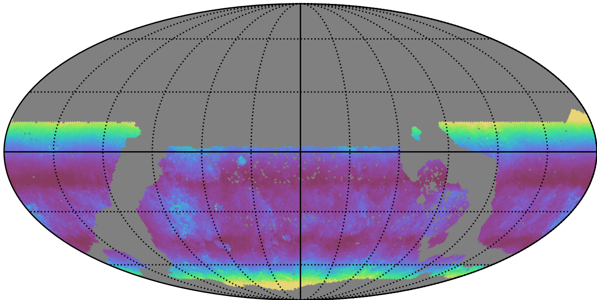
too_elab_r8_d2_ugrizy_v3.4_10yrs WFD g band: Median airmass
