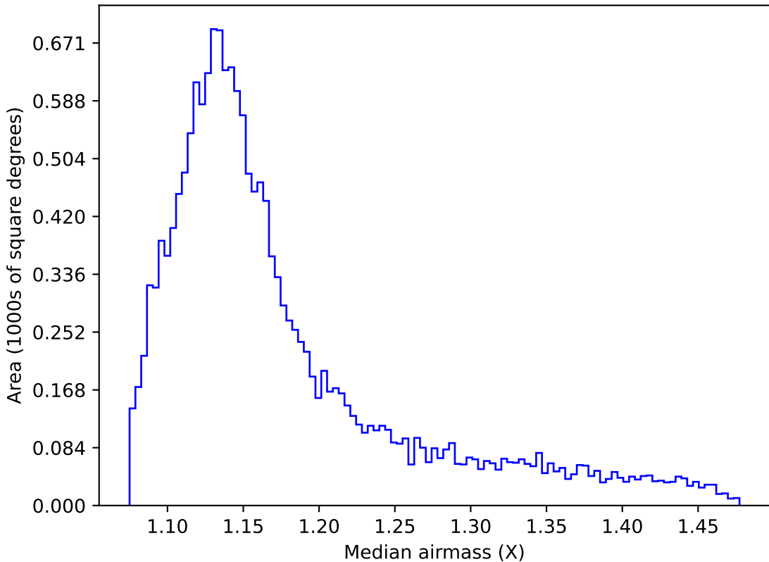
too_elab_r8_d2_ugrizy_v3.4_10yrs WFD g band: Median airmass
