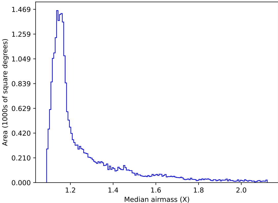
too_elab_r8_d2_ugrizy_v3.4_10yrs All sky z band: Median airmass
