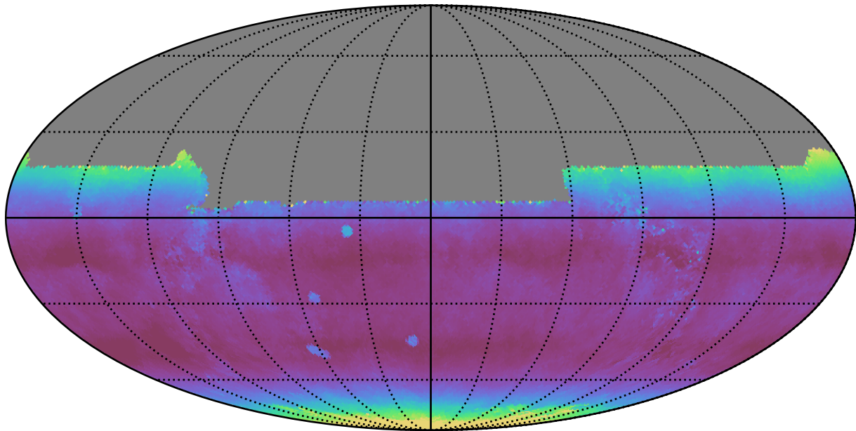
too_elab_r8_d2_ugrizy_v3.4_10yrs All sky y band: Median airmass
