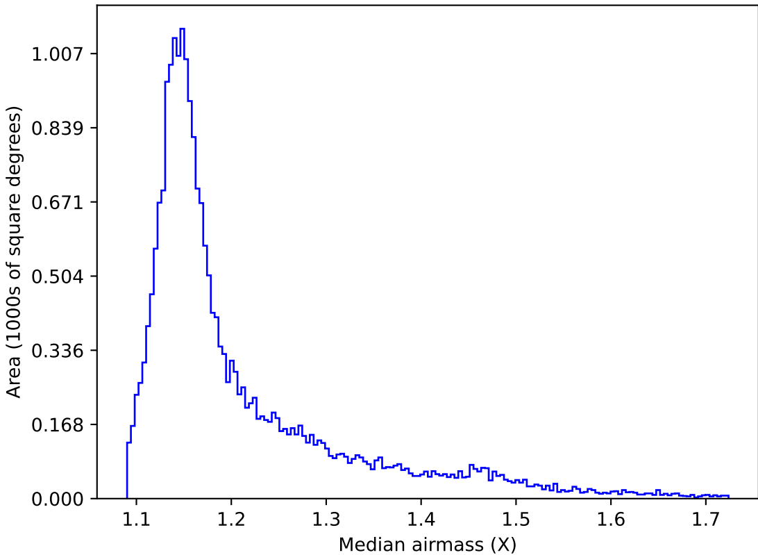
too_elab_r8_d2_ugrizy_v3.4_10yrs All sky y band: Median airmass
