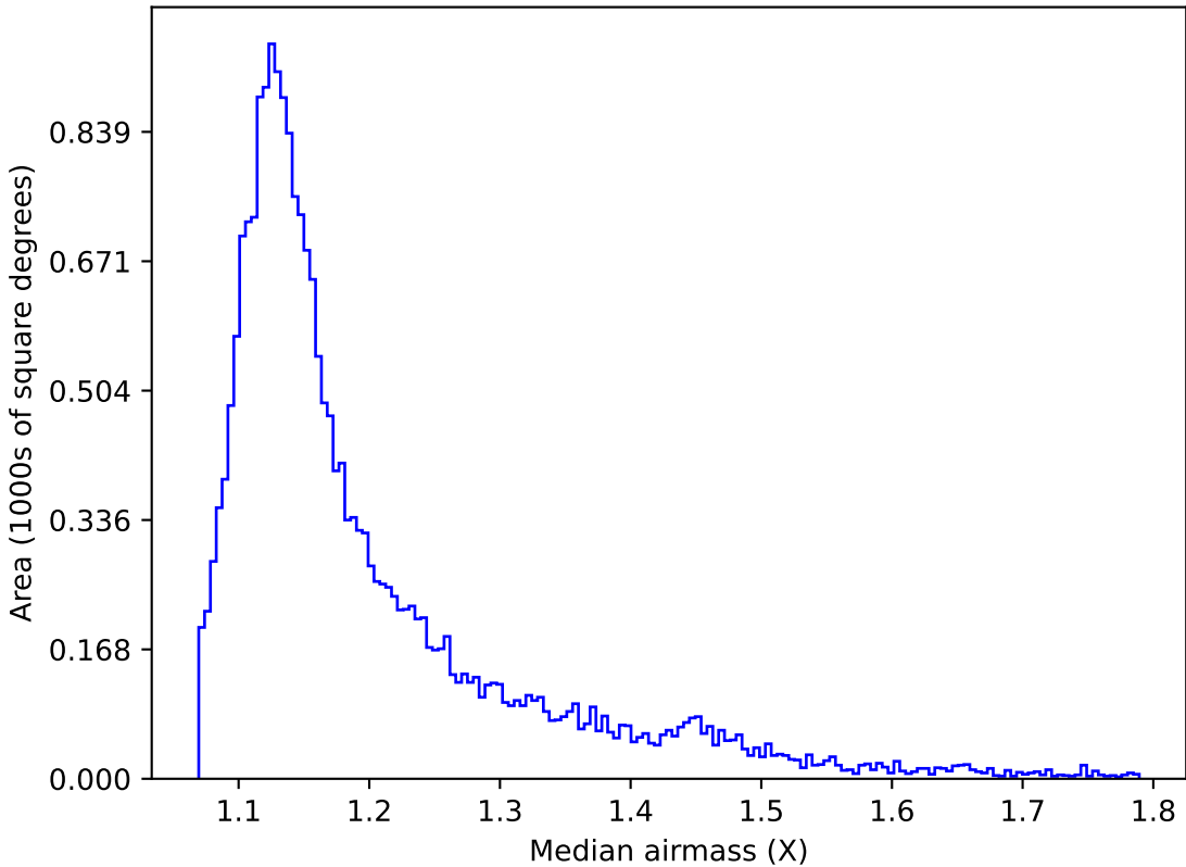
too_elab_r8_d2_ugrizy_v3.4_10yrs All sky u band: Median airmass
