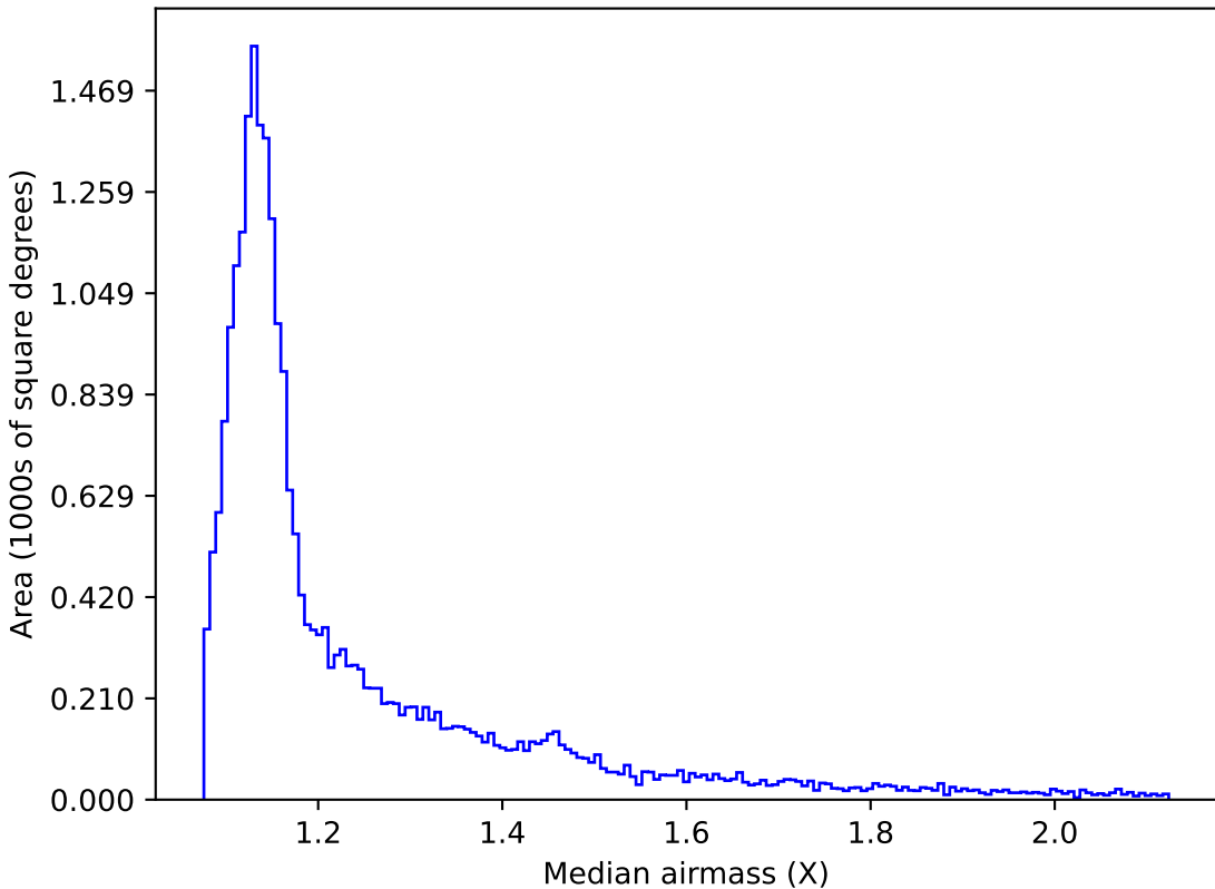
too_elab_r8_d2_ugrizy_v3.4_10yrs All sky r band: Median airmass
