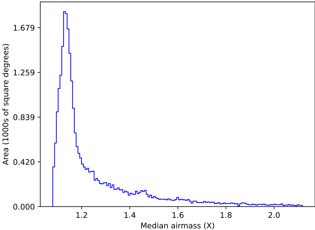
too_elab_r8_d2_ugrizy_v3.4_10yrs All sky i band: Median airmass
