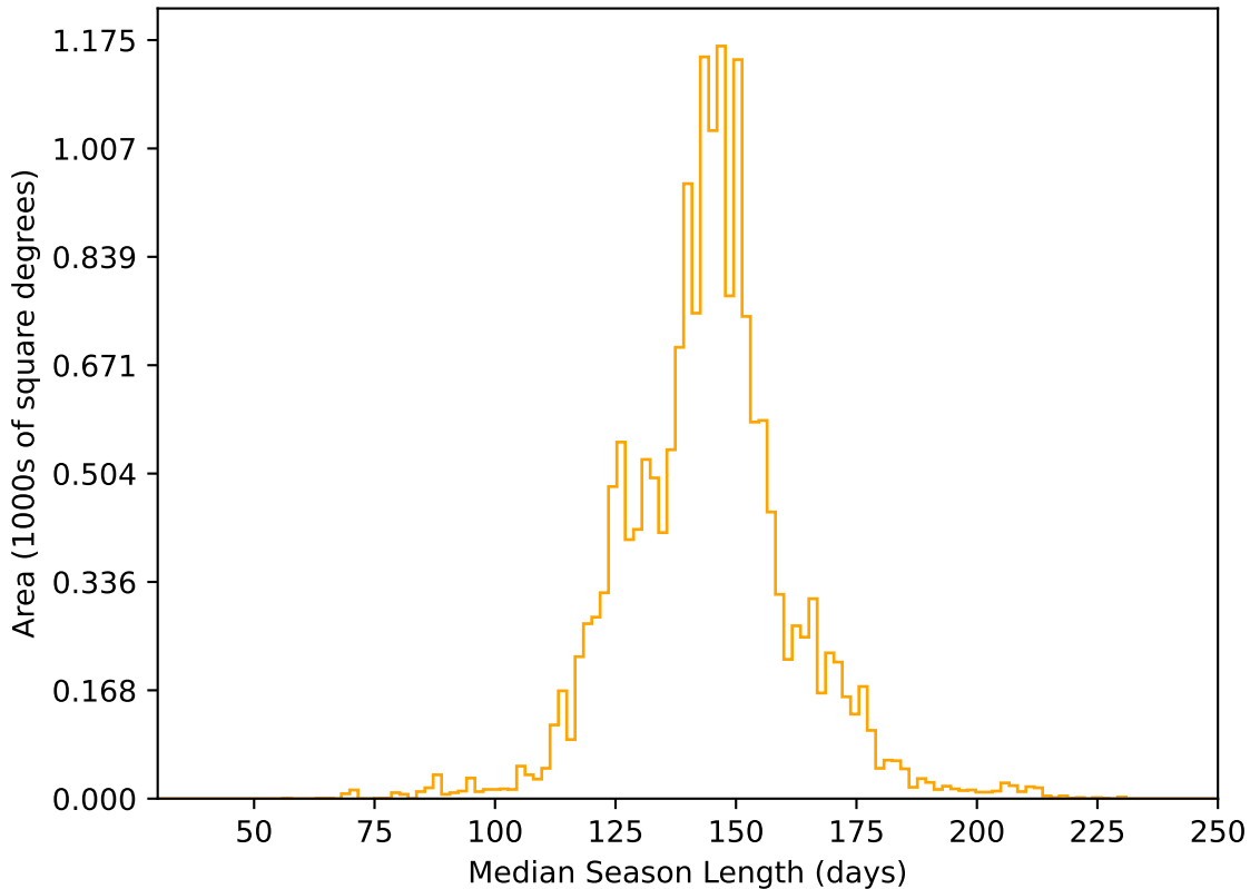
too_elab_r8_d2_ugrizy_v3.4_10yrs WFD r band: Median Season Length
