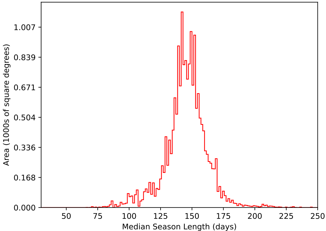
too_elab_r8_d2_ugrizy_v3.4_10yrs WFD i band: Median Season Length
