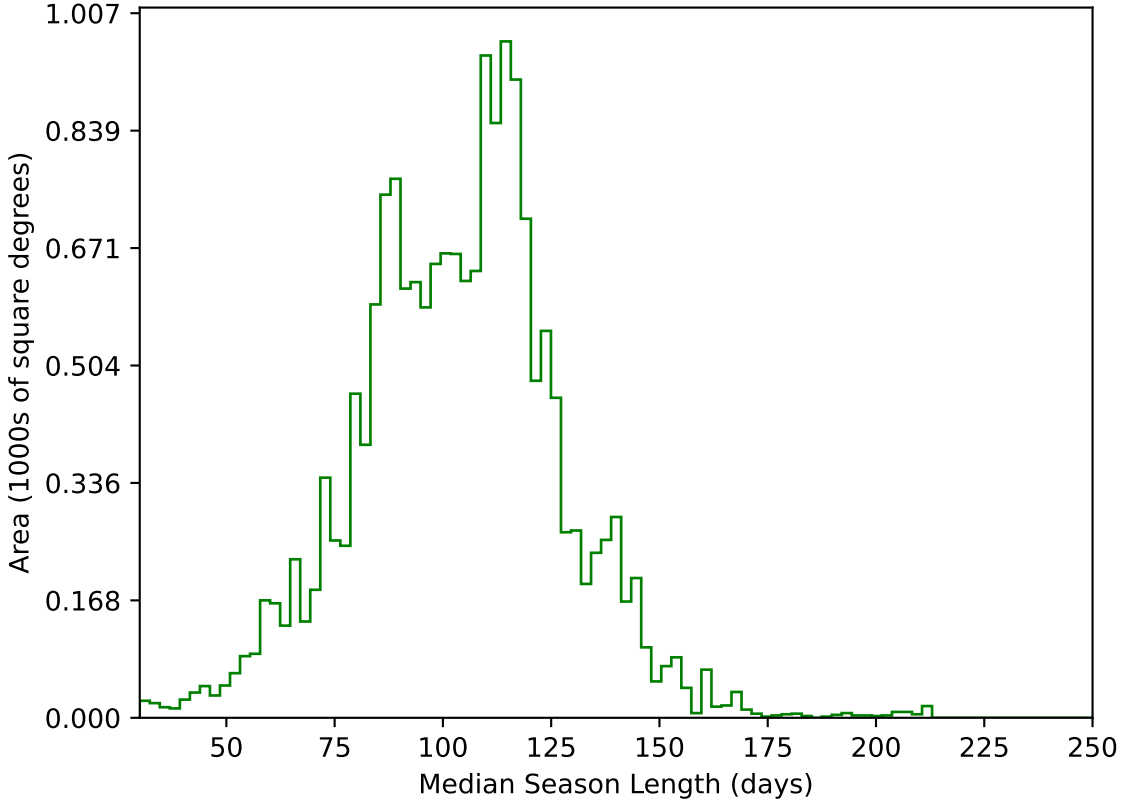
too_elab_r8_d2_ugrizy_v3.4_10yrs WFD g band: Median Season Length
